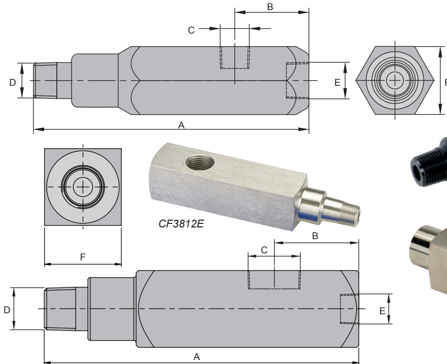
CF3812
