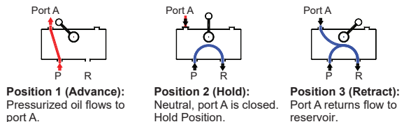
Figure 4 - Flowpath of the valve positions and operations for Model P2301M.
