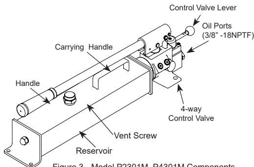
Figure 3 - Model P2301M, P4301M Components
